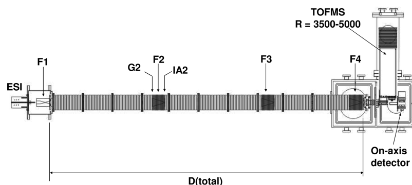
Figure 1. Schematic of a prototype IMS-IMS-IMS-TOF instrument, 43,44 where “F” corresponds to an ion funnel, “G” is the selection gate, and “IA” is an ion activation region. See text for more details.
