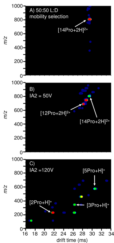
Figure 3. A narrow distribution of [14\text{Pro}+2\text{H}]^{2+} cluster formed from the 50:50 L/D solution is (a) mobility selected and activated with (b) 50 V and (c) 120 V in the IA2 region. At the relatively low activation voltage (50 V), the [14\text{Pro}+2\text{H}]^{2+} cluster evaporates neutral monomers. At the higher activation voltage (120 V), the doubly charged clusters fission to produce singly charged proline clusters.
