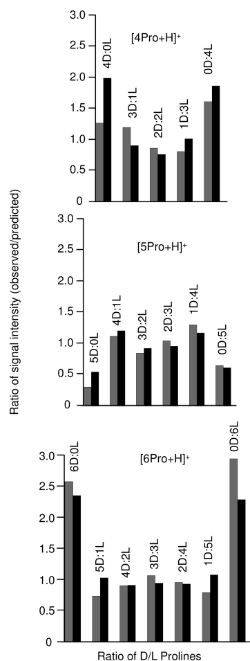
Figure 5. Ratio of the observed to predicted (statistical) intensities for the proline clusters: [4\text{Pro}+\text{H}]^+ , [5\text{Pro}+\text{H}]^+ , and [6\text{Pro}+\text{H}]^+ , where the x axis refers to the number of L/D prolines in clusters formed from the 50:50 D- and L- [(\text{HN}(\text{CD}_2)_3\text{CD})\text{COOH}] proline mixture. Gray bar graphs represent data obtained for the singly charged clusters formed by CID. Black bar graphs represent data obtained for the singly charged clusters formed during electrospray.
