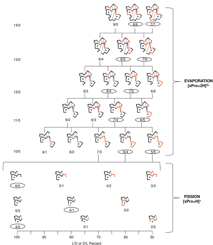
Figure 6. A hypothetical schematic showing the dissociation scheme of the mixed L/D [14\text{Pro}+2\text{H}]^{2+} cluster. The residue evaporation and ion fission regions of the fragmentation process are labeled. Cluster ion compositions are designated by the numbers of L- and D-proline residues as “L/D”. Composition degeneracies are not designated (see text for details). Circled compositions represent preferred fragmentation pathways (see preferred fragments in Figures 4 and 5).
